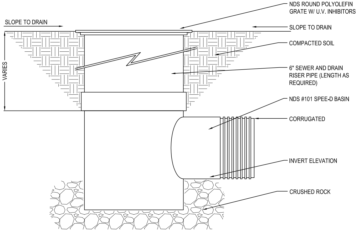
SECTION
