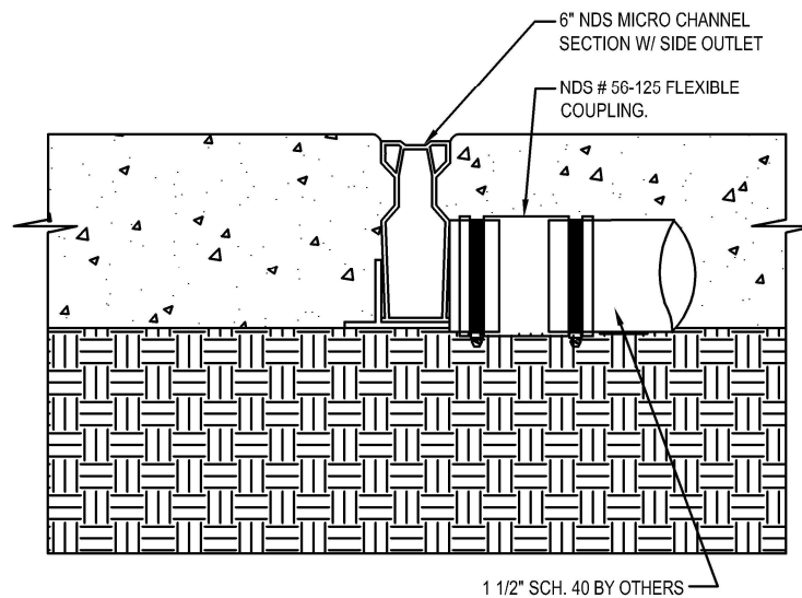
SIDE OUTLET WITH FLEXIBLE COUPLING
