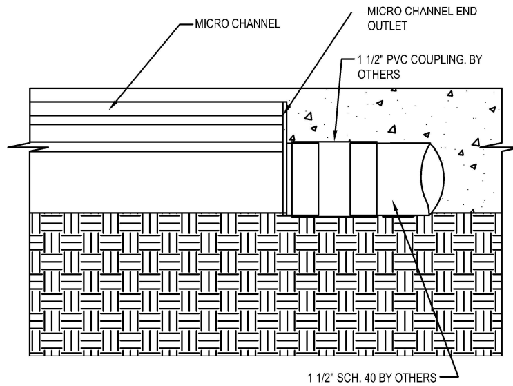
END OUTLET WITH PVC COUPLING
