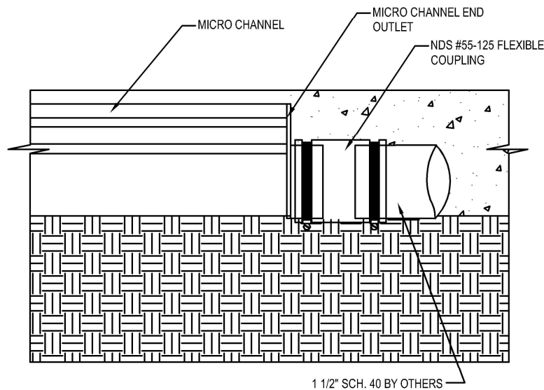
END OUTLET WITH FLEXIBLE COUPLING
