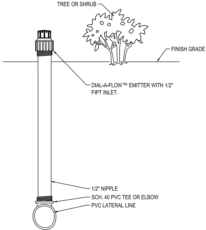
SECTION
