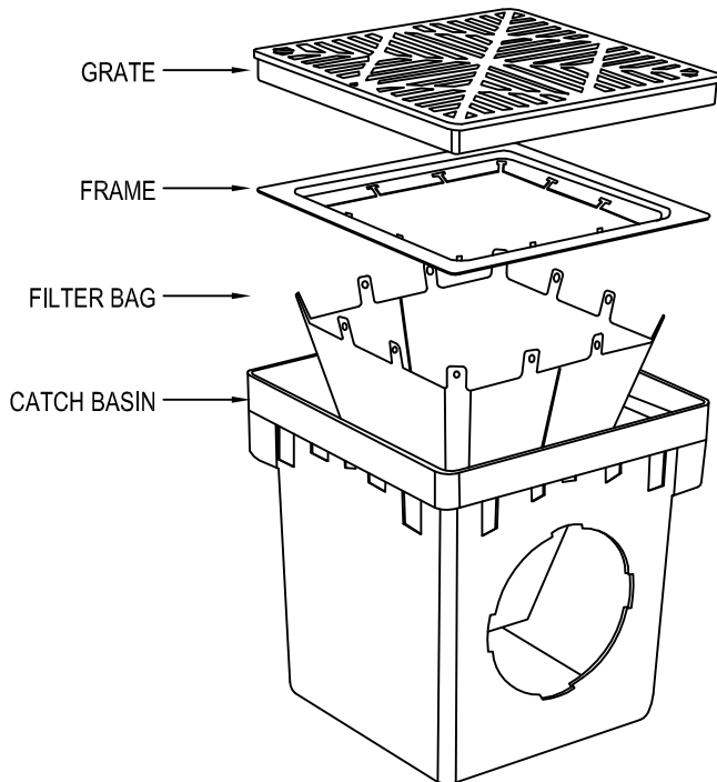
ISOMETRIC
