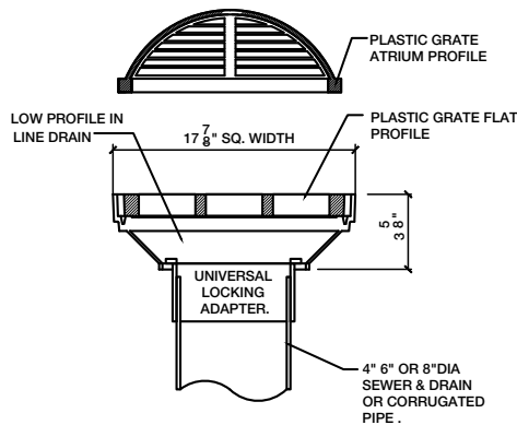
Example: Adapter with Dome Grate
