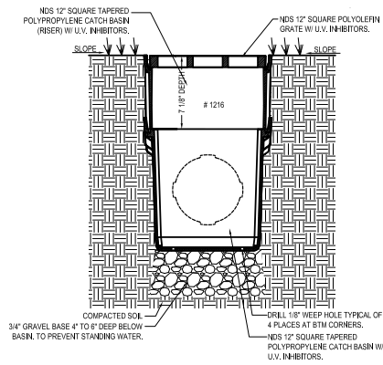
Example: 12" Catch Basin with Single Riser
