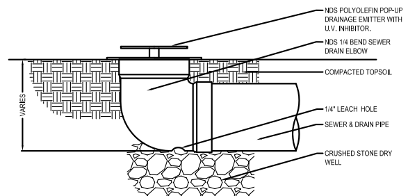
Example: Fitting and Pop-up Emitter
