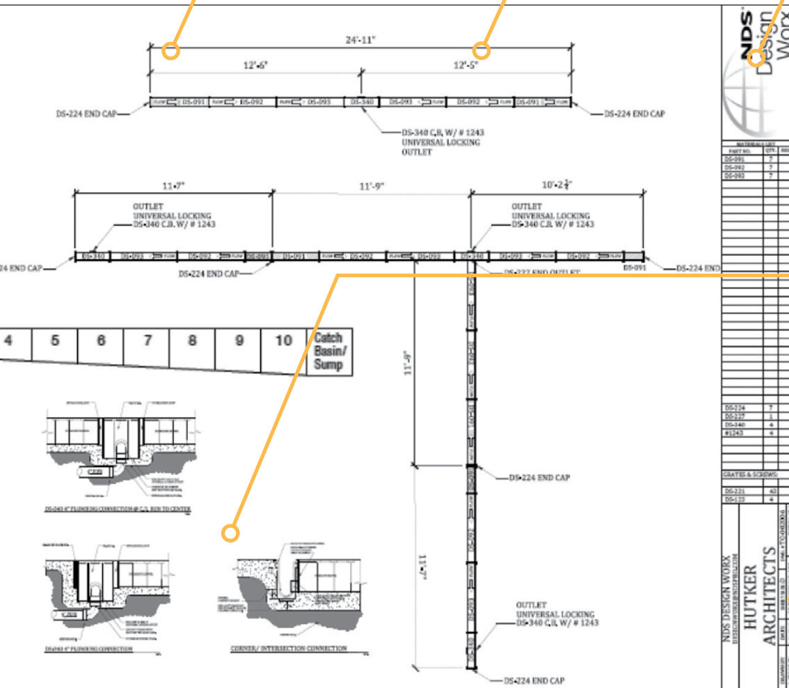
Installation details
