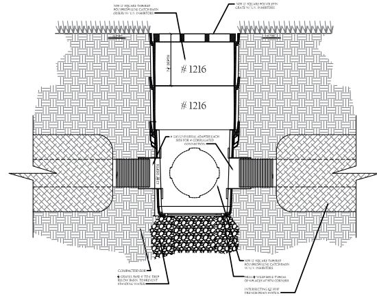
Example: 12" Catch Basin with Two Risers
