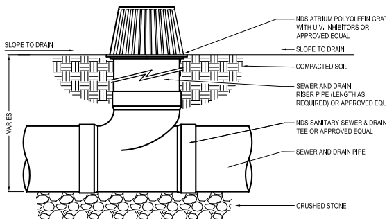
Example: Fitting and Dome Grate
