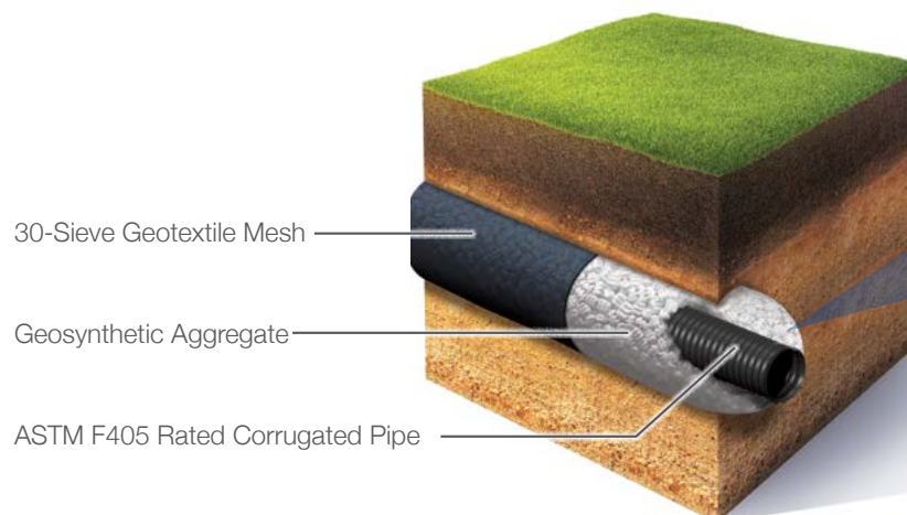
Behind Wall or Foundation
