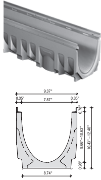
Pro 200 Galvanized Steel Trench Drain
